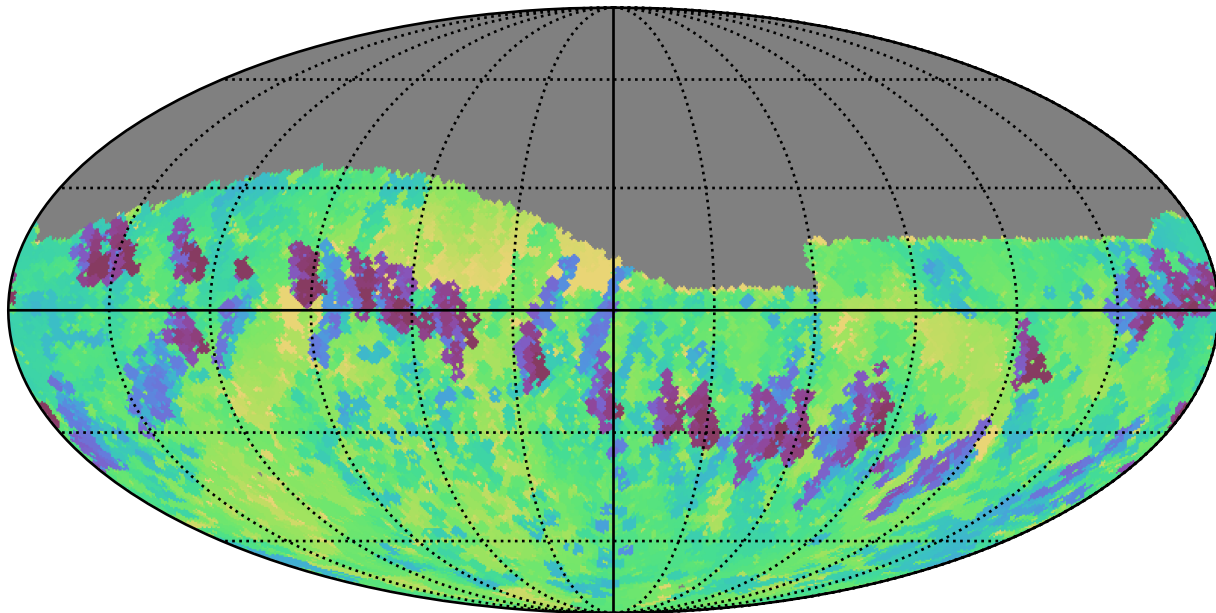
too_combined_s0.5_v3.4_10yrs Yr 1 z band: Min skyBrightness
