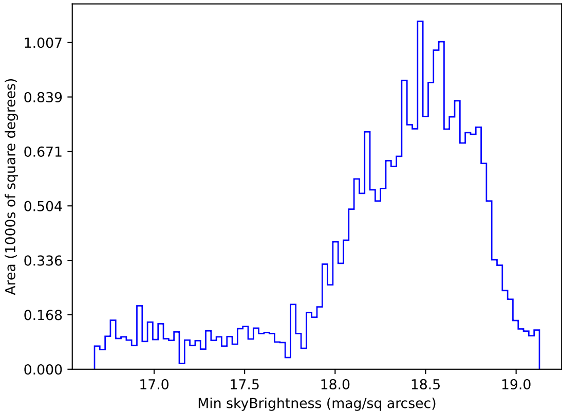
too_combined_s0.5_v3.4_10yrs Yr 1 z band: Min skyBrightness
