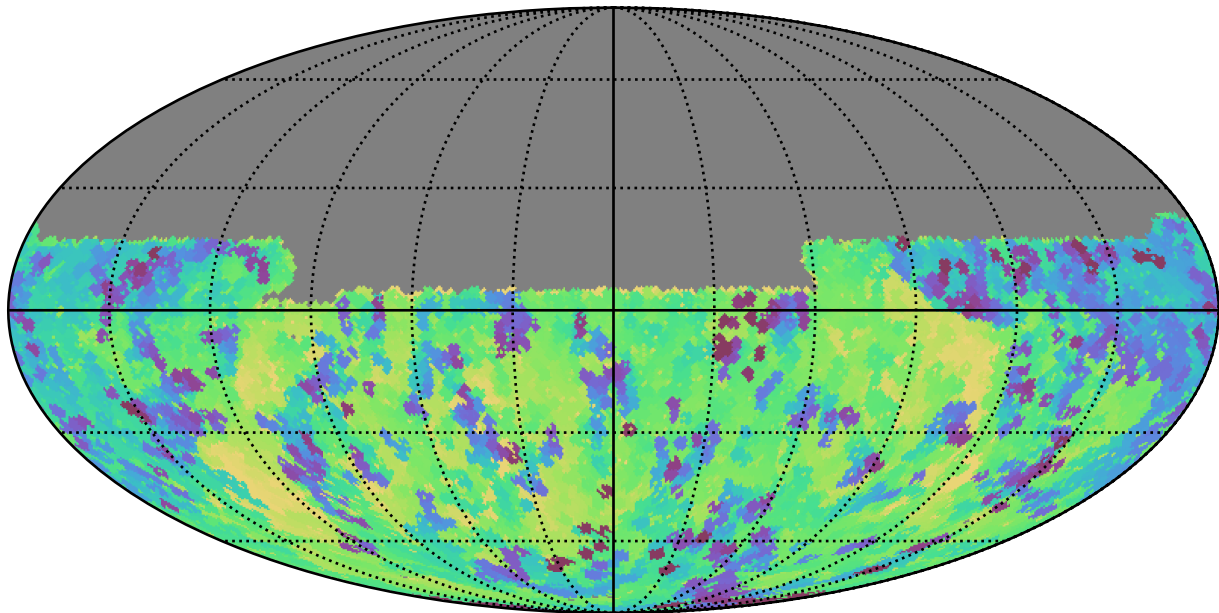
too_combined_s0.5_v3.4_10yrs Yr 1 y band: Min skyBrightness
