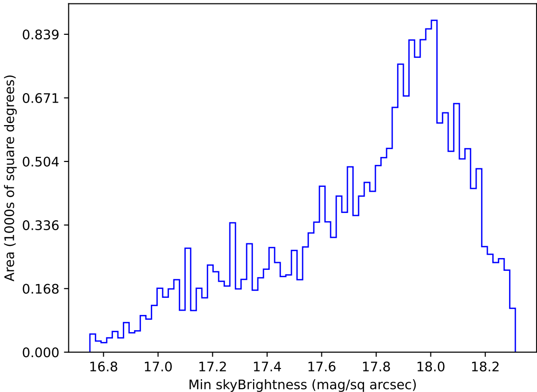
too_combined_s0.5_v3.4_10yrs Yr 1 y band: Min skyBrightness
