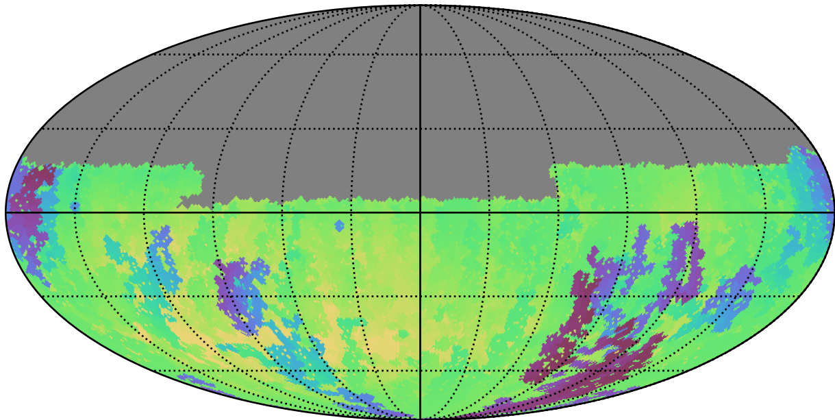
too_combined_s0.5_v3.4_10yrs Yr 1 u band: Min skyBrightness
