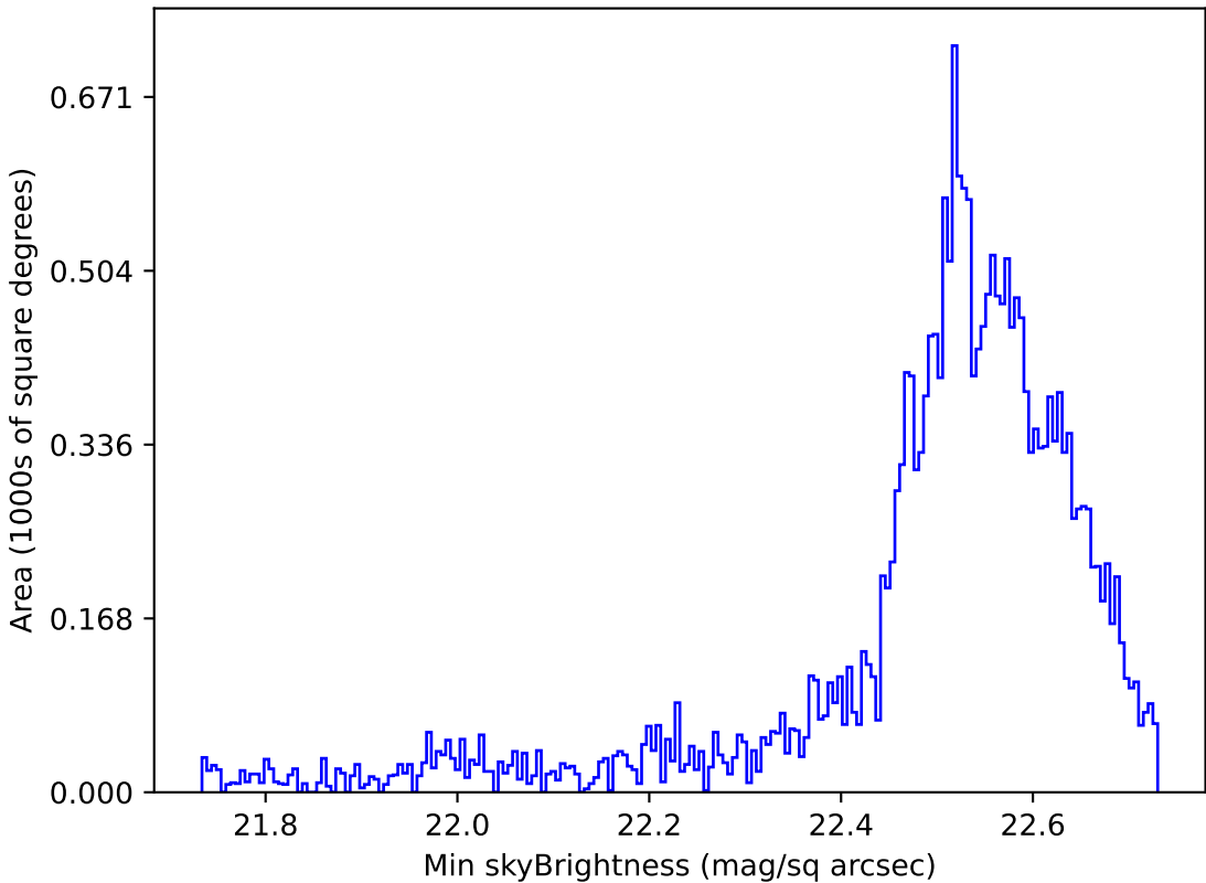
too_combined_s0.5_v3.4_10yrs Yr 1 u band: Min skyBrightness
