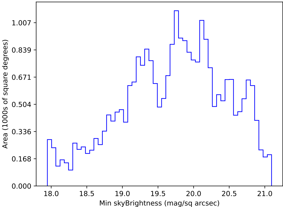
too_combined_s0.5_v3.4_10yrs Yr 1 r band: Min skyBrightness
