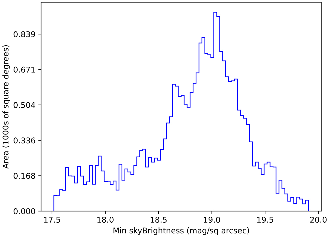
too_combined_s0.5_v3.4_10yrs Yr 1 i band: Min skyBrightness
