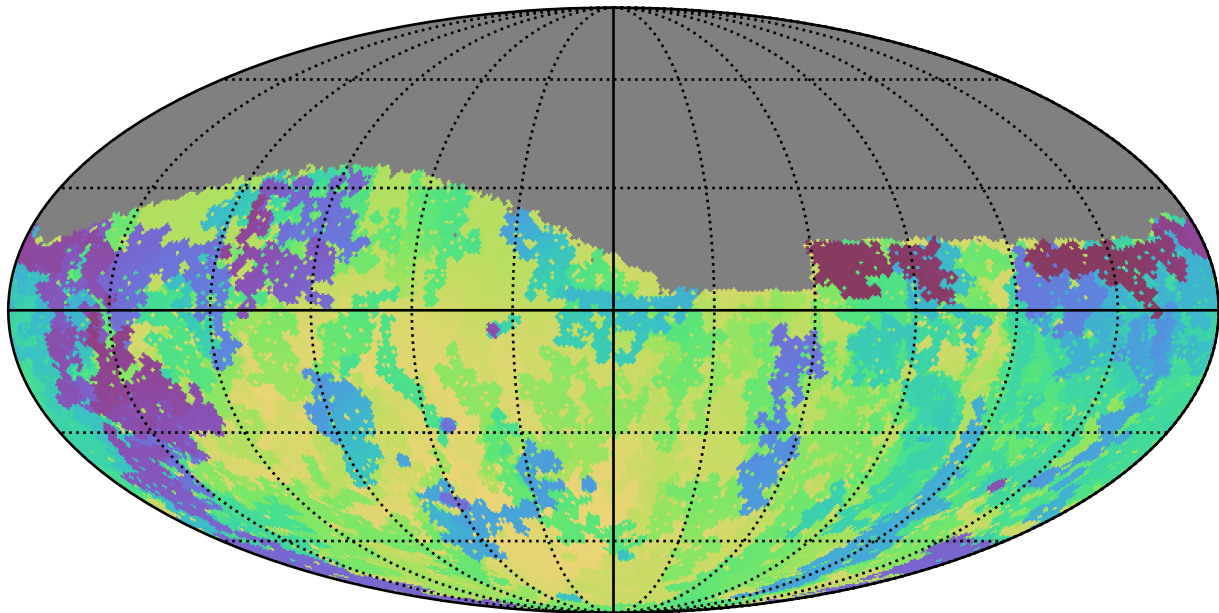
too_combined_s0.5_v3.4_10yrs Yr 1 g band: Min skyBrightness
