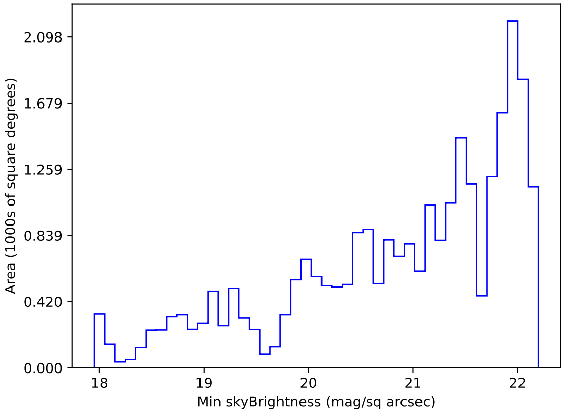
too_combined_s0.5_v3.4_10yrs Yr 1 g band: Min skyBrightness
