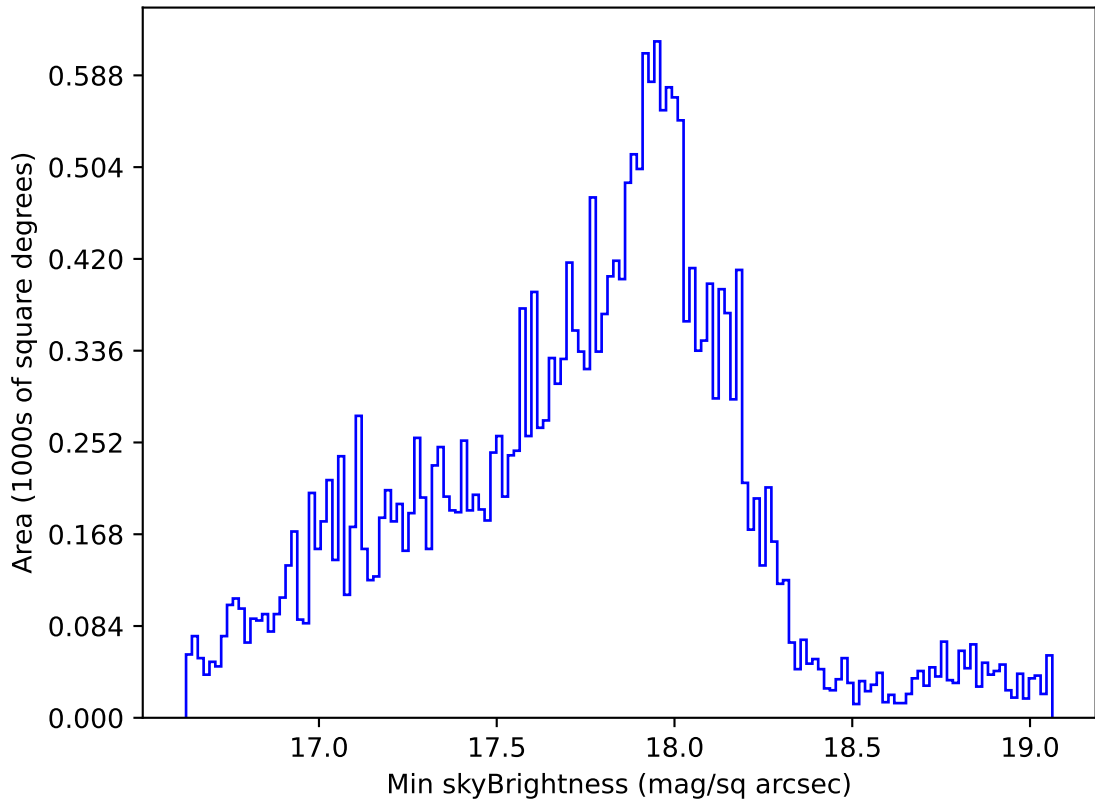
too_combined_s0.5_v3.4_10yrs Yr 1 all bands: Min skyBrightness
