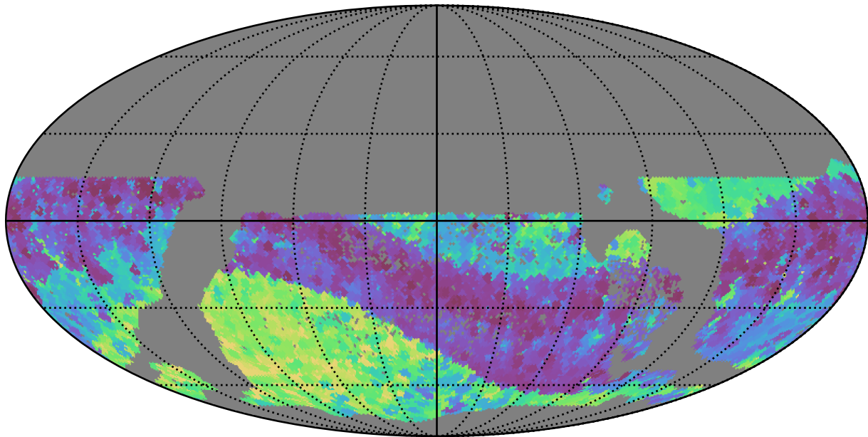
too_combined_s0.5_v3.4_10yrs WFD z band: Min skyBrightness
