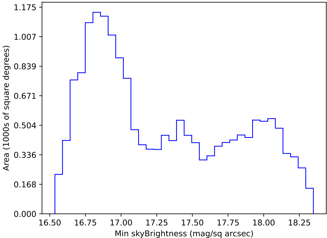
too_combined_s0.5_v3.4_10yrs WFD z band: Min skyBrightness
