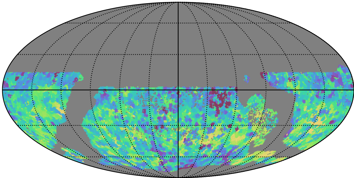
too_combined_s0.5_v3.4_10yrs WFD y band: Min skyBrightness
