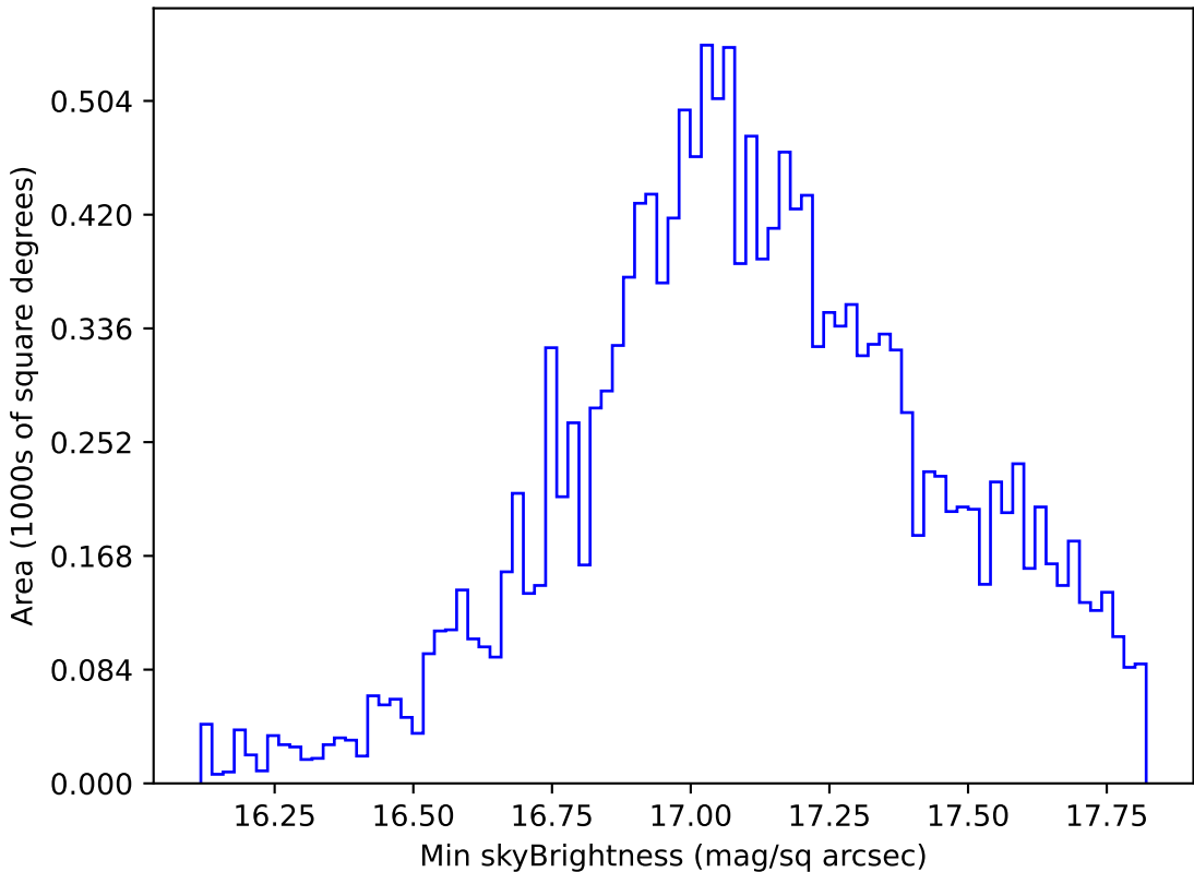
too_combined_s0.5_v3.4_10yrs WFD y band: Min skyBrightness
