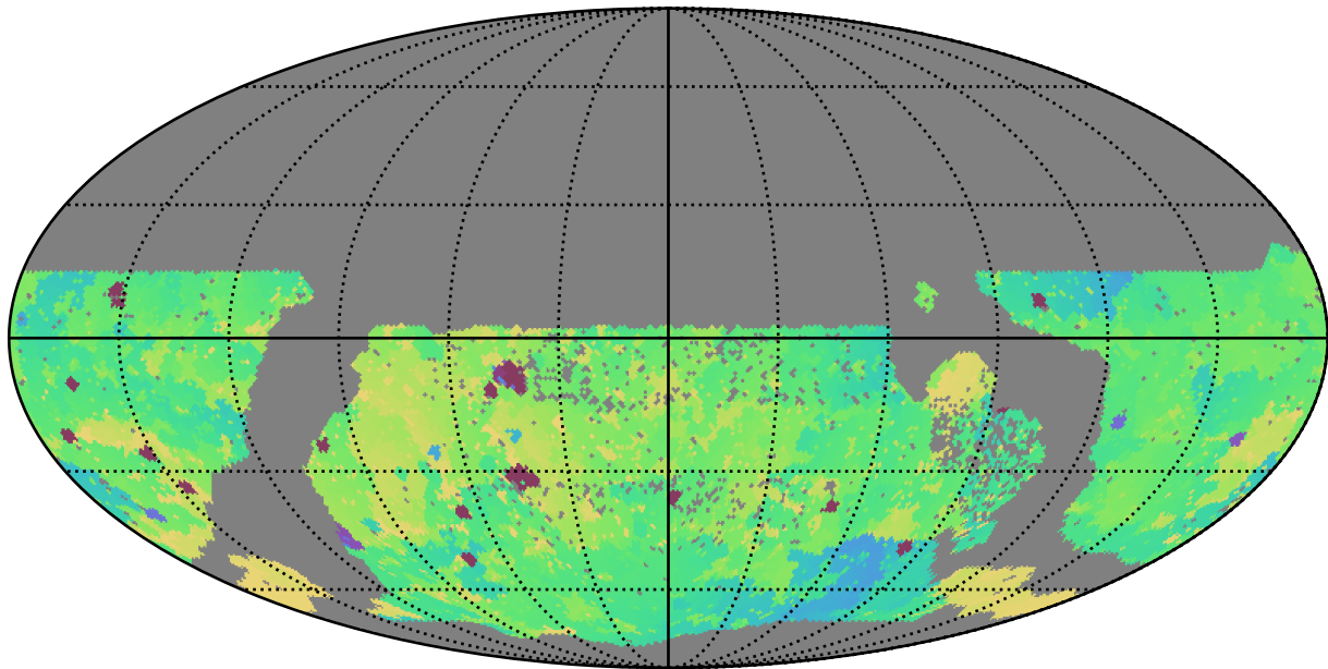
too_combined_s0.5_v3.4_10yrs WFD u band: Min skyBrightness
