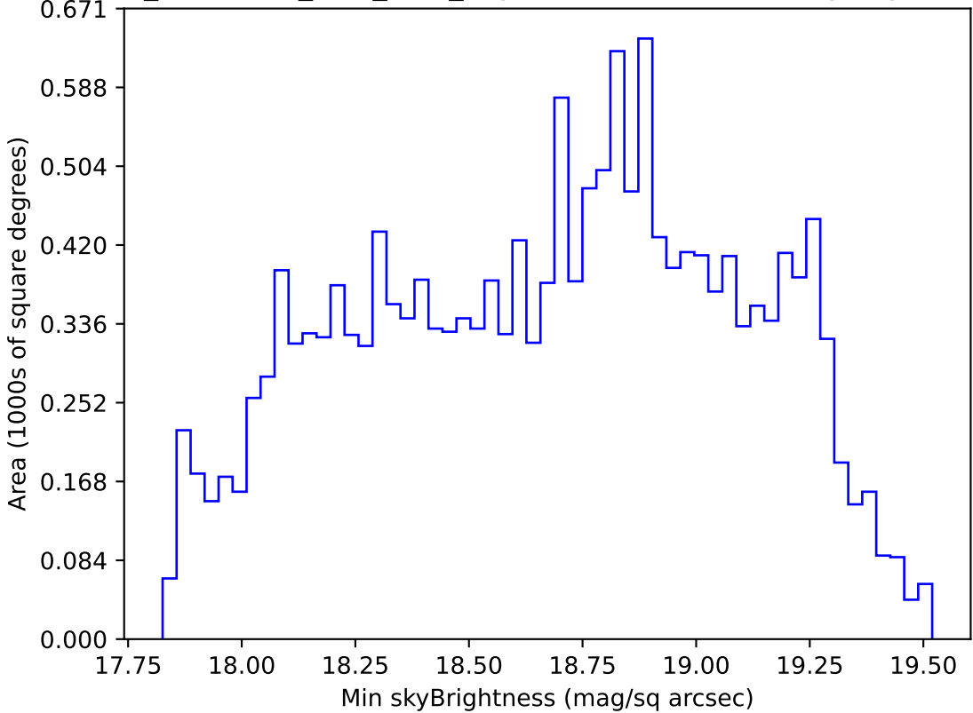
too_combined_s0.5_v3.4_10yrs WFD r band: Min skyBrightness
