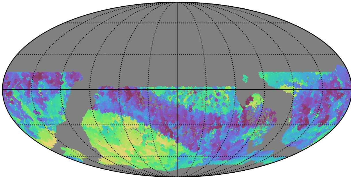
too_combined_s0.5_v3.4_10yrs WFD i band: Min skyBrightness
