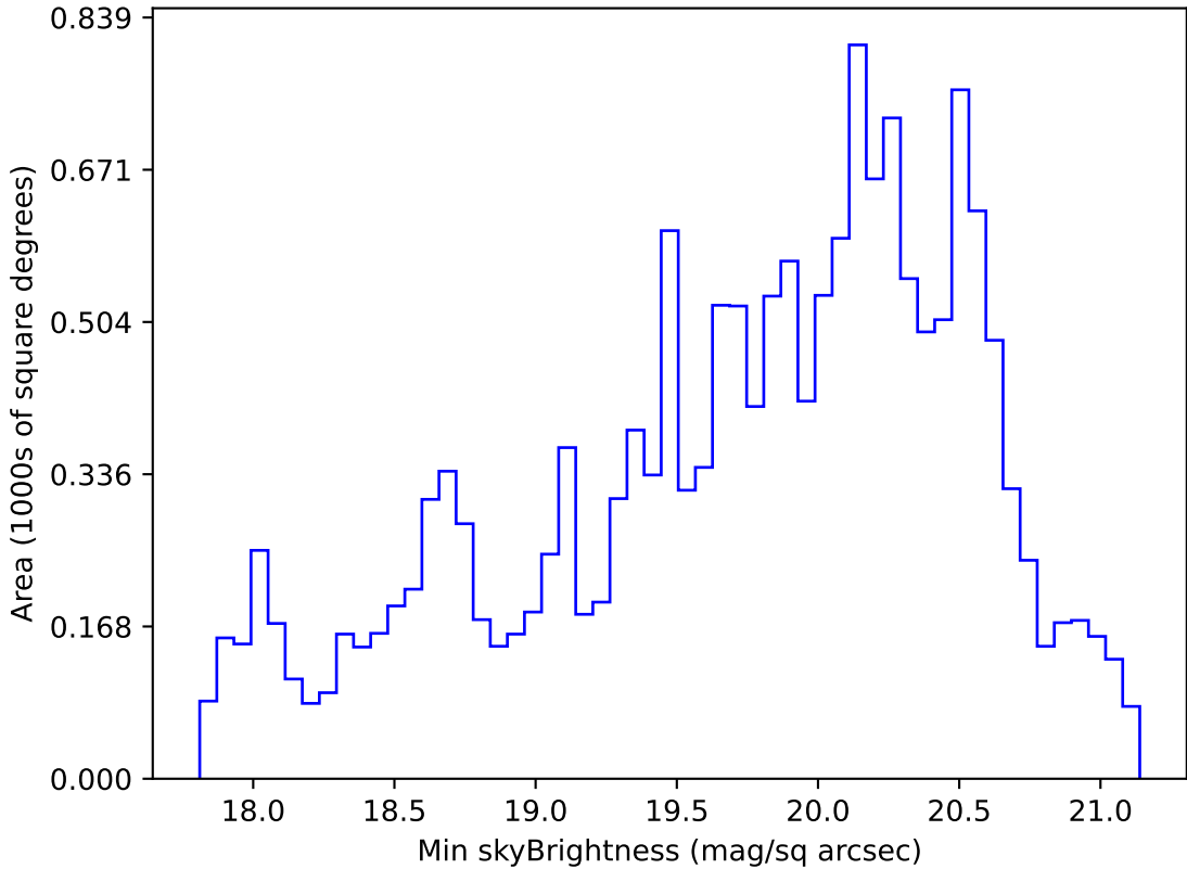
too_combined_s0.5_v3.4_10yrs WFD g band: Min skyBrightness
