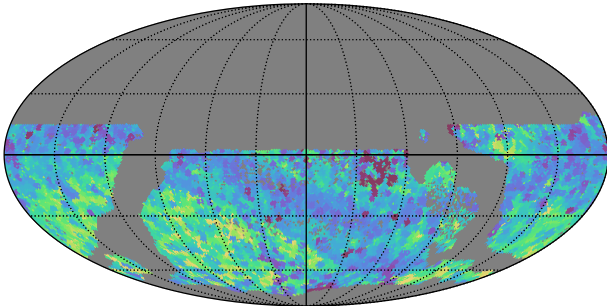
too_combined_s0.5_v3.4_10yrs WFD all bands: Min skyBrightness
