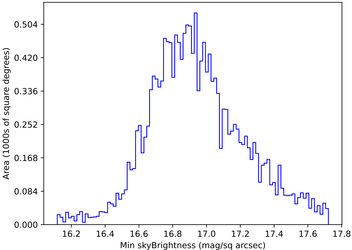
too_combined_s0.5_v3.4_10yrs WFD all bands: Min skyBrightness
