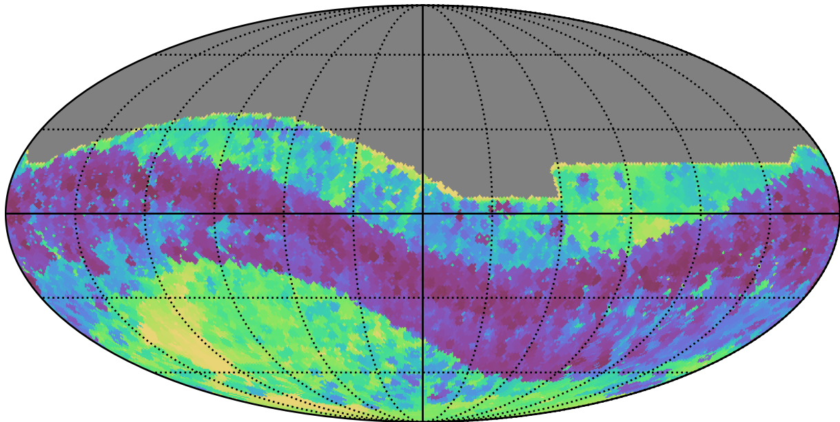
too_combined_s0.5_v3.4_10yrs All sky z band: Min skyBrightness
