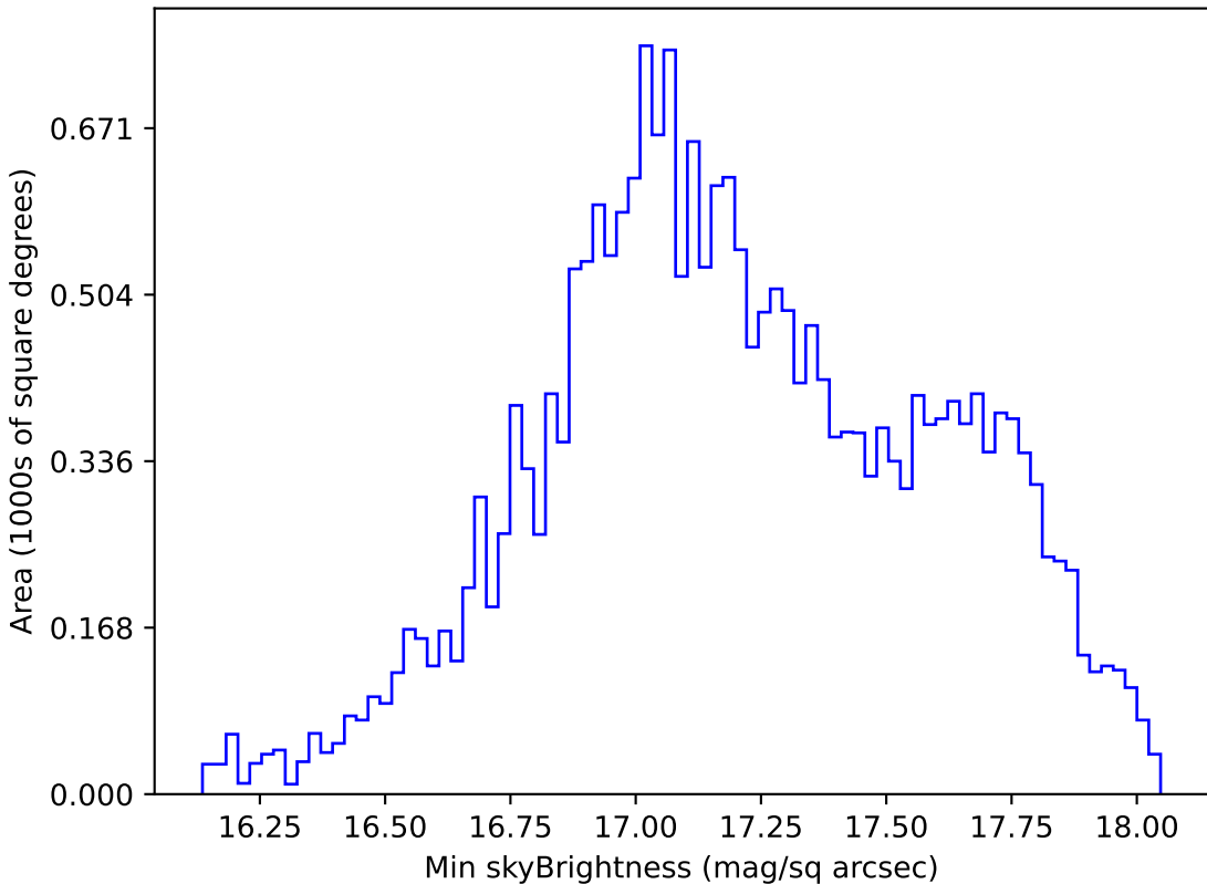
too_combined_s0.5_v3.4_10yrs All sky y band: Min skyBrightness
