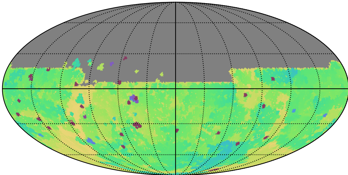
too_combined_s0.5_v3.4_10yrs All sky u band: Min skyBrightness
