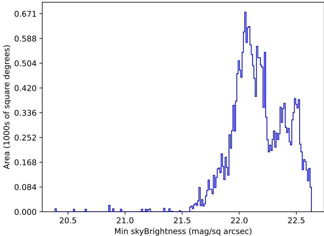
too_combined_s0.5_v3.4_10yrs All sky u band: Min skyBrightness
