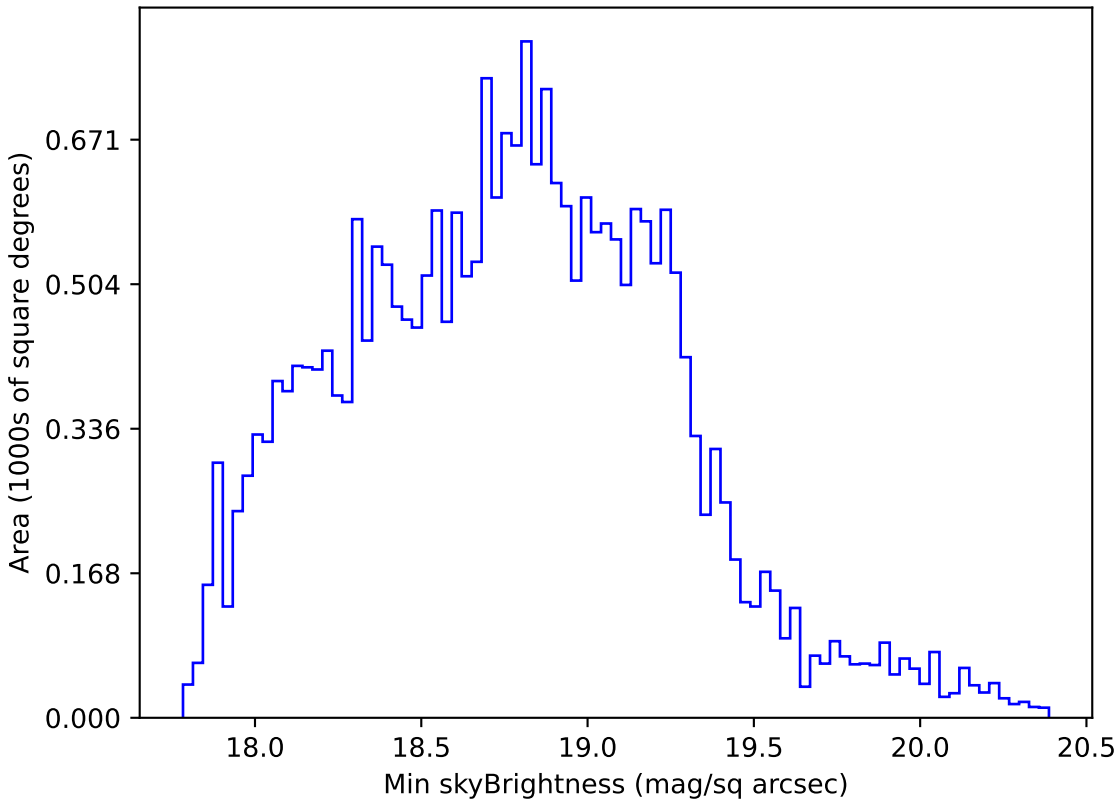
too_combined_s0.5_v3.4_10yrs All sky r band: Min skyBrightness
