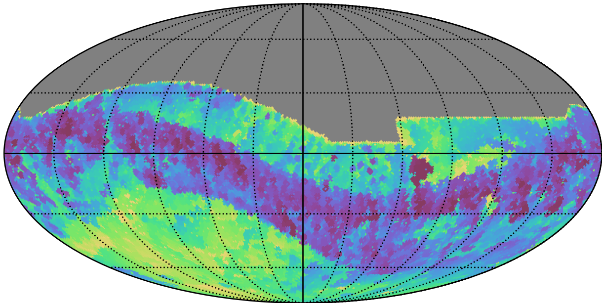
too_combined_s0.5_v3.4_10yrs All sky i band: Min skyBrightness
