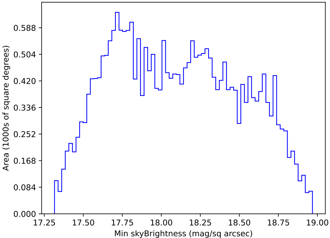
too_combined_s0.5_v3.4_10yrs All sky i band: Min skyBrightness
