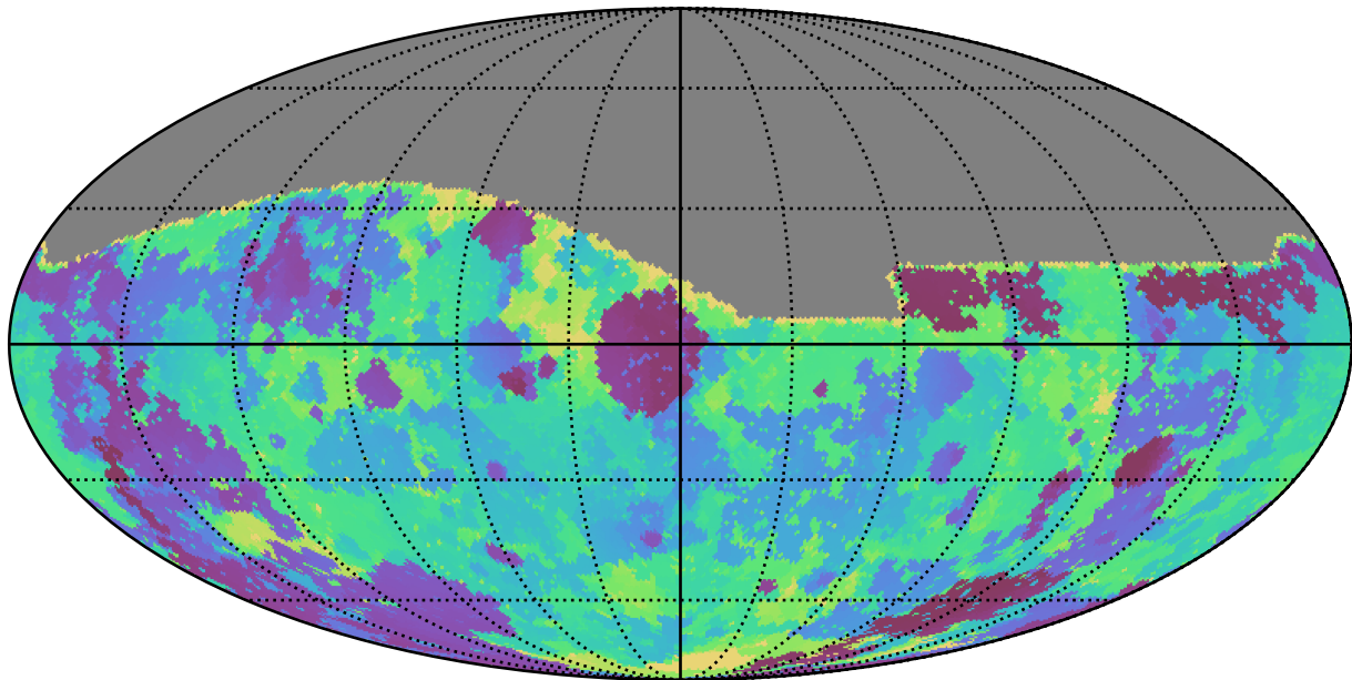
too_combined_s0.5_v3.4_10yrs All sky g band: Min skyBrightness
