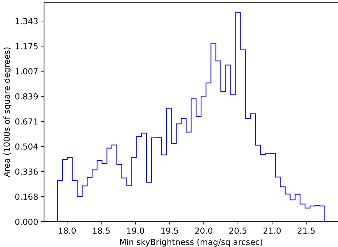
too_combined_s0.5_v3.4_10yrs All sky g band: Min skyBrightness
