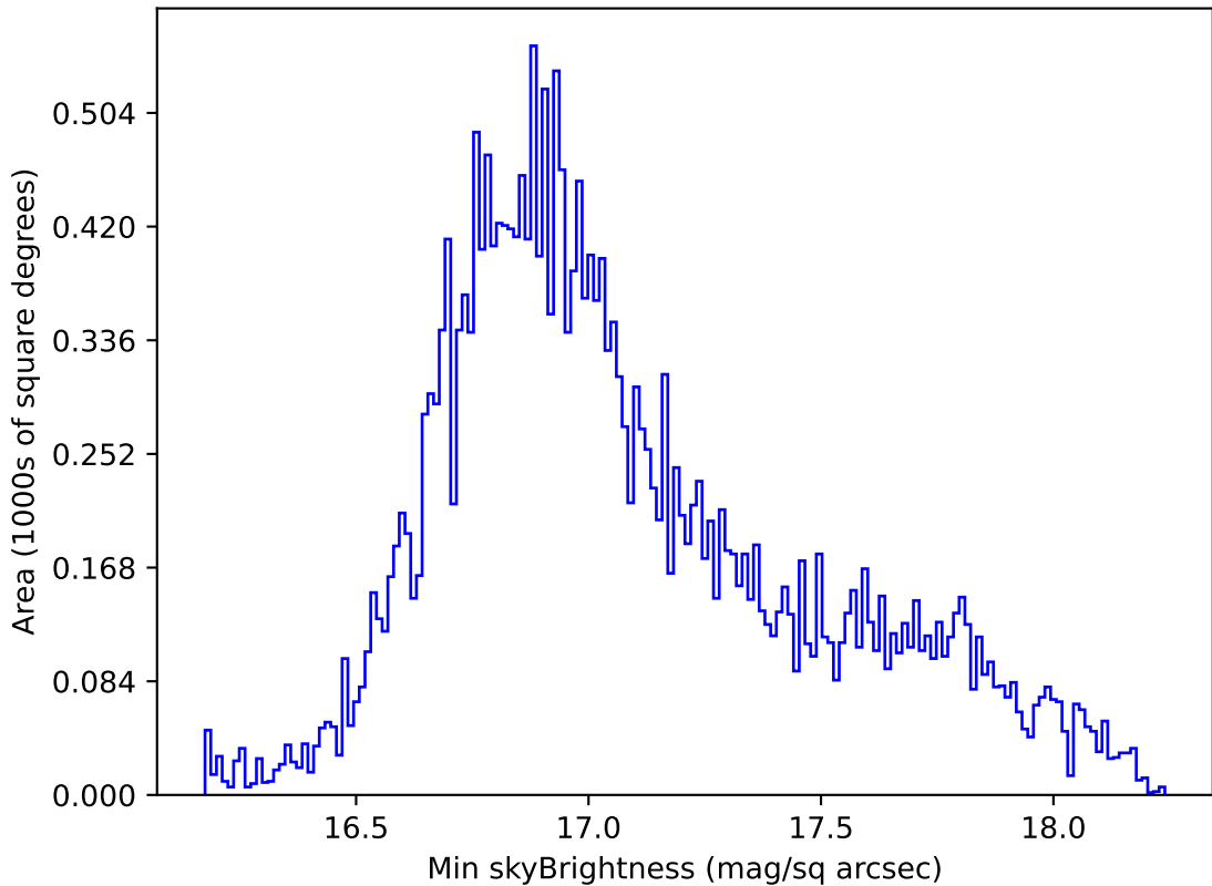
too_combined_s0.5_v3.4_10yrs All sky all bands: Min skyBrightness
