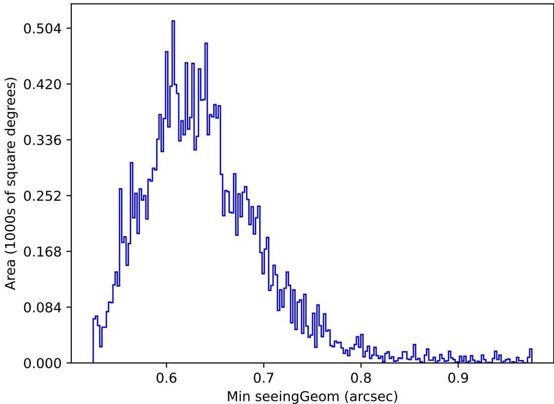
too_combined_s0.5_v3.4_10yrs Yr 1 y band: Min seeingGeom
