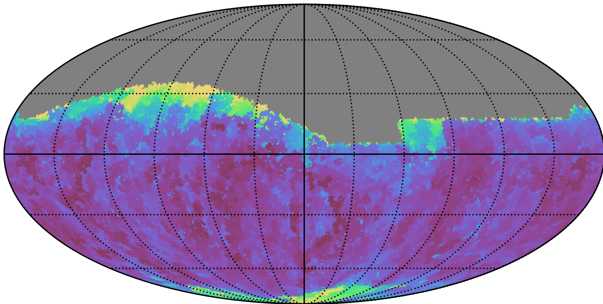
too_combined_s0.5_v3.4_10yrs Yr 1 r band: Min seeingGeom
