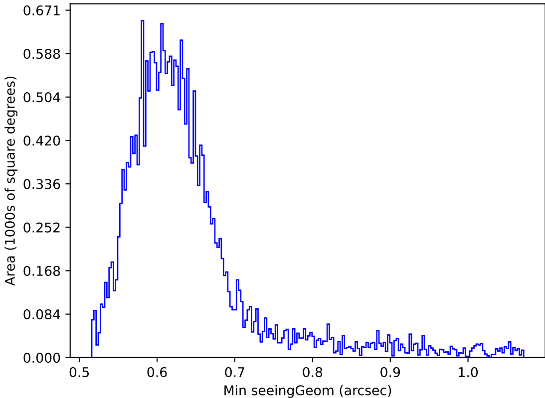
too_combined_s0.5_v3.4_10yrs Yr 1 r band: Min seeingGeom
