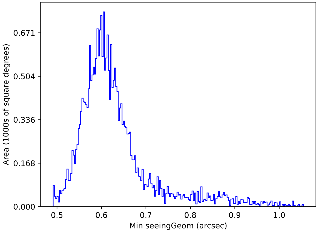
too_combined_s0.5_v3.4_10yrs Yr 1 i band: Min seeingGeom
