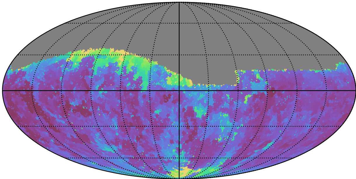
too_combined_s0.5_v3.4_10yrs Yr 1 g band: Min seeingGeom
