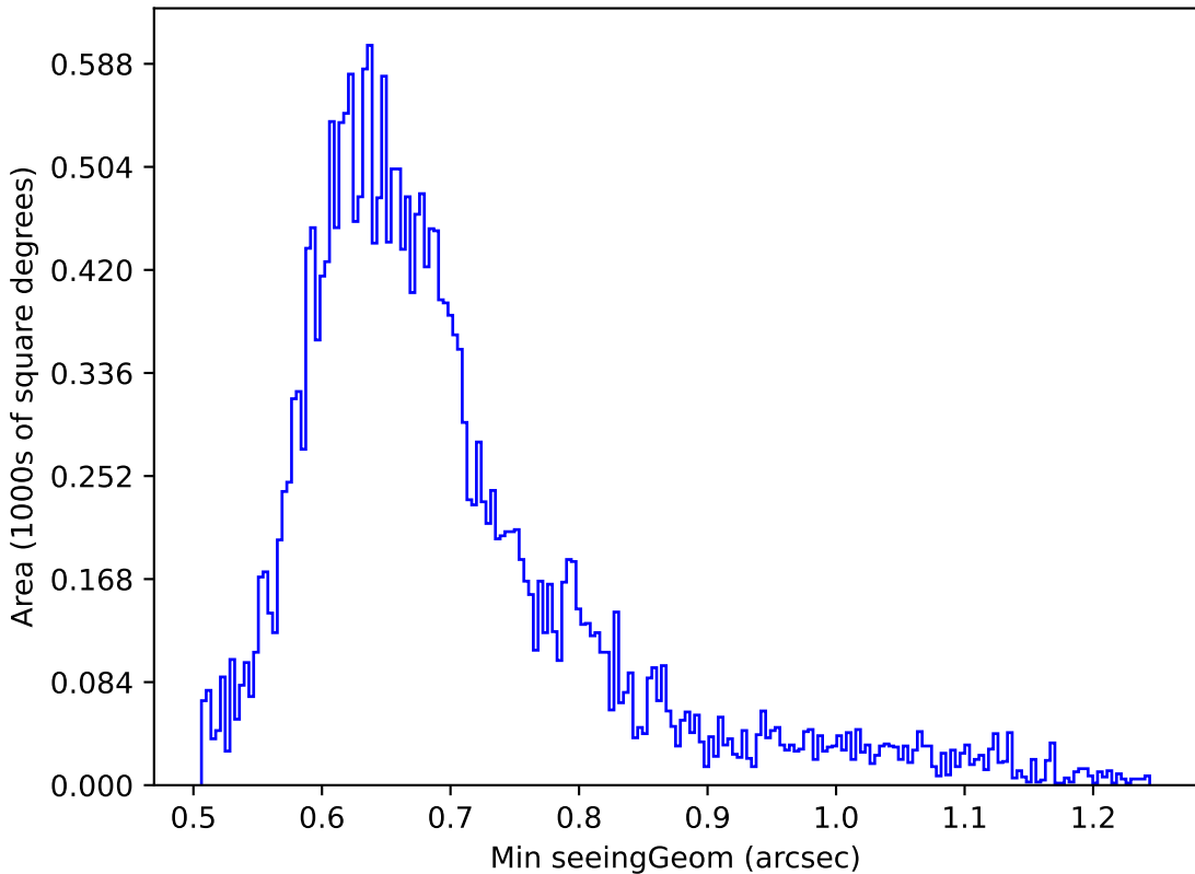
too_combined_s0.5_v3.4_10yrs Yr 1 g band: Min seeingGeom
