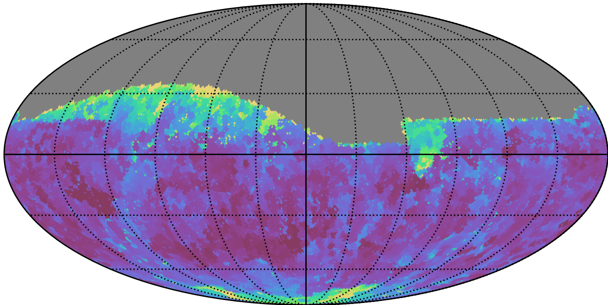
too_combined_s0.5_v3.4_10yrs Yr 1 z band: Min seeingEff
