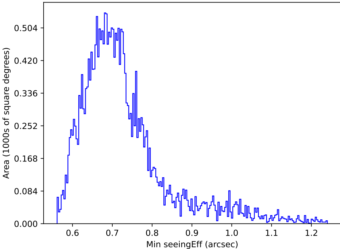
too_combined_s0.5_v3.4_10yrs Yr 1 z band: Min seeingEff
