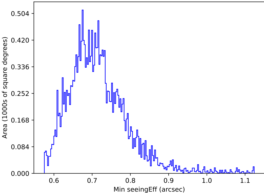
too_combined_s0.5_v3.4_10yrs Yr 1 y band: Min seeingEff
