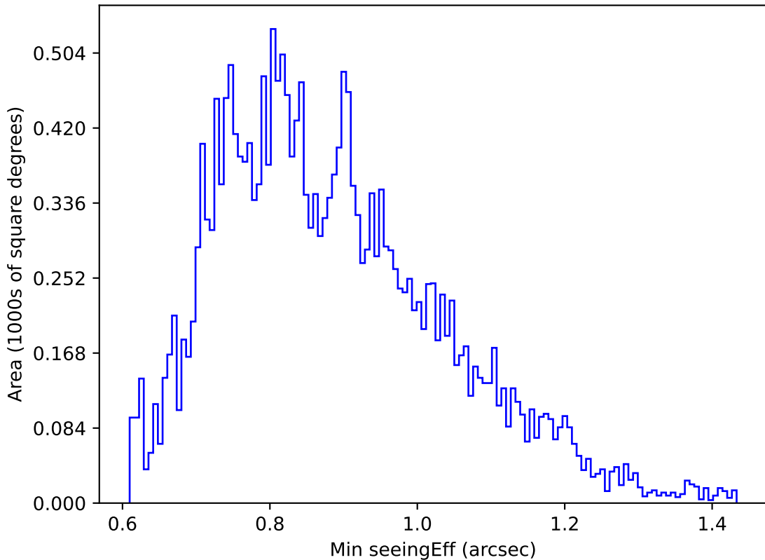
too_combined_s0.5_v3.4_10yrs Yr 1 u band: Min seeingEff
