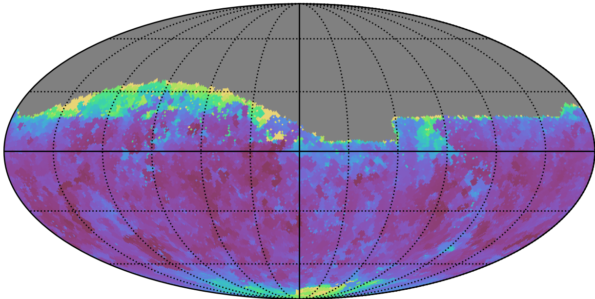
too_combined_s0.5_v3.4_10yrs Yr 1 r band: Min seeingEff
