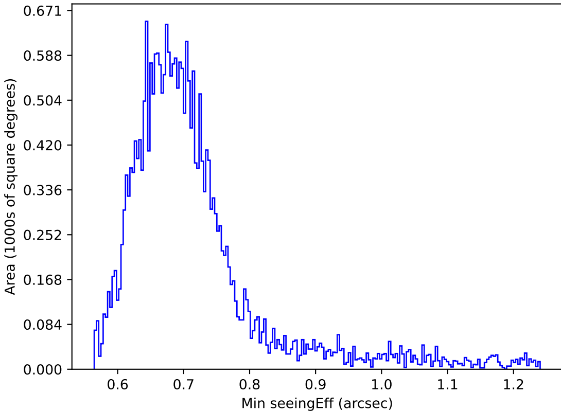
too_combined_s0.5_v3.4_10yrs Yr 1 r band: Min seeingEff
