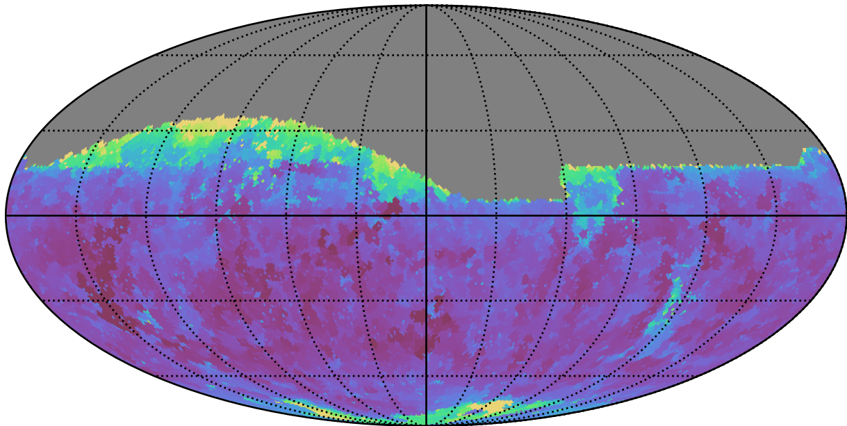
too_combined_s0.5_v3.4_10yrs Yr 1 i band: Min seeingEff
