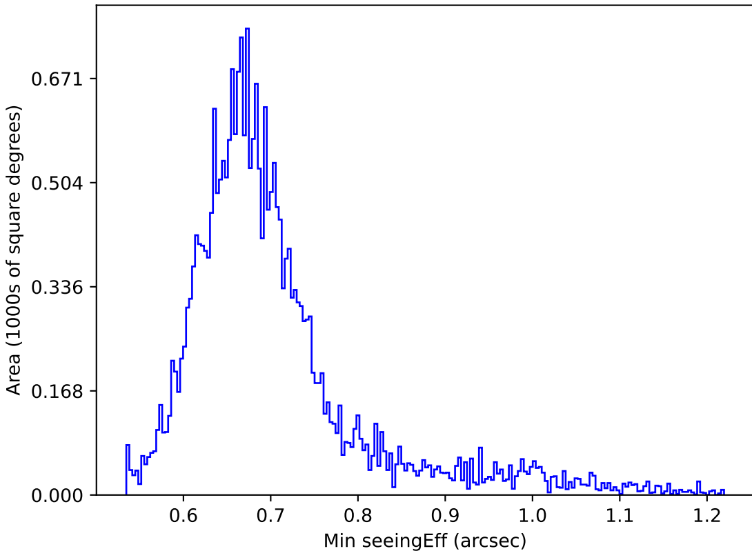
too_combined_s0.5_v3.4_10yrs Yr 1 i band: Min seeingEff
