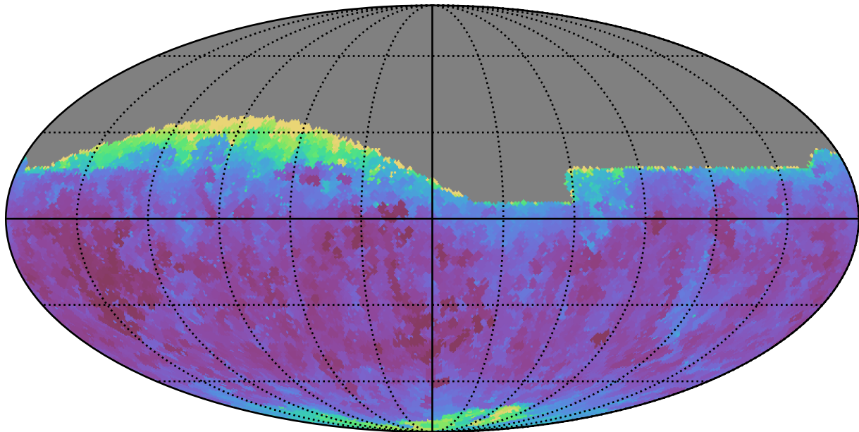
too_combined_s0.5_v3.4_10yrs Yr 1 all bands: Min seeingEff
