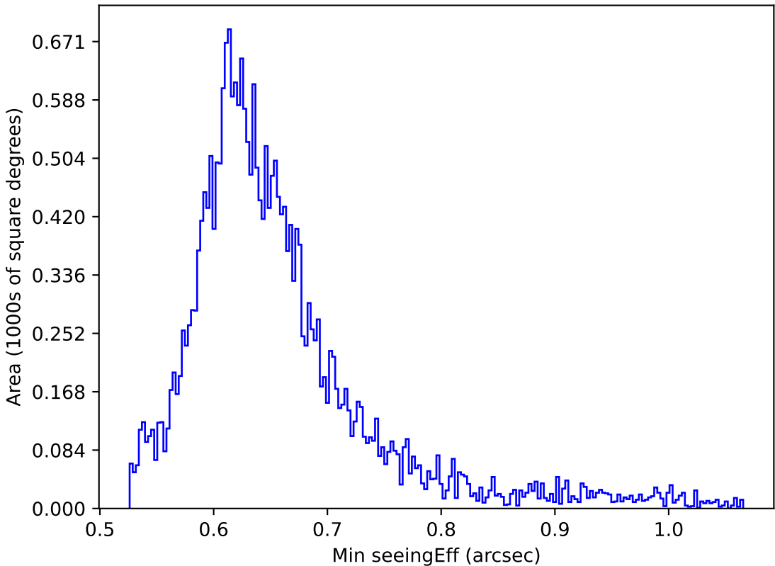
too_combined_s0.5_v3.4_10yrs Yr 1 all bands: Min seeingEff
