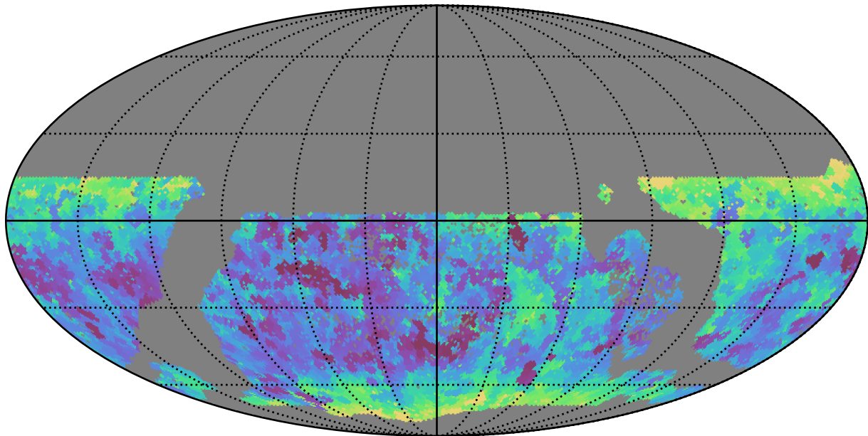
too_combined_s0.5_v3.4_10yrs WFD z band: Min seeingEff
