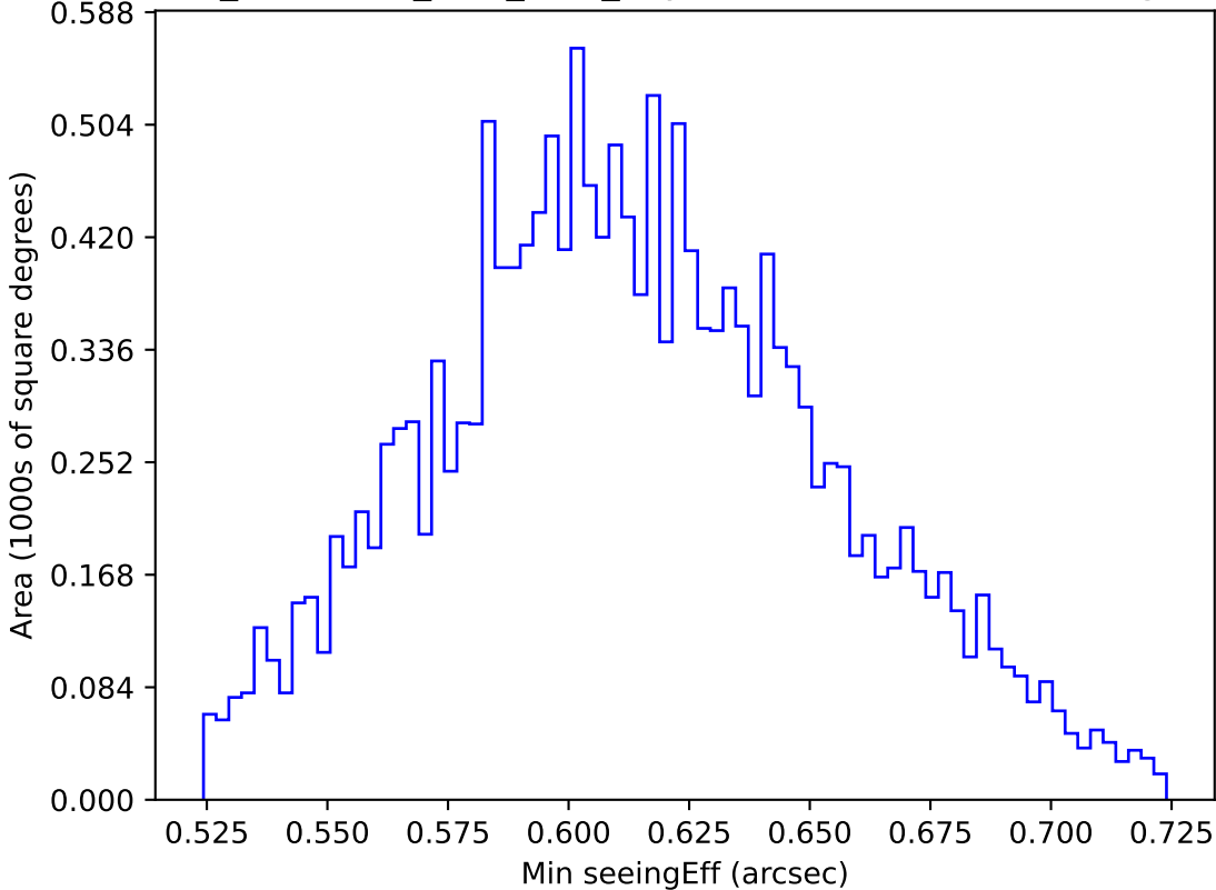
too_combined_s0.5_v3.4_10yrs WFD z band: Min seeingEff
