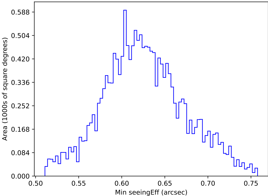
too_combined_s0.5_v3.4_10yrs WFD y band: Min seeingEff
